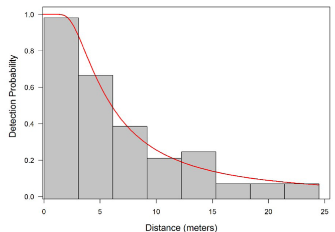
Figure 3. Detection curve of West Indian manatees ( Trichechus manatus ) in the Timonha-Ubatuba Estuarine System, Northeastern Brazil, given by the hazard-rate model (red line). The columns show the relative frequency of manatee detections in the study.
