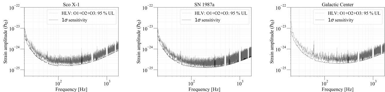
FIG. 6. Upper limits on the dimensionless strain amplitude h_0 , using the data from three observing runs of LIGO-Virgo detectors, at the 95% confidence level for the narrow band radiometer search are indicated by the gray bands for Scorpius X-1 (left), SN 1987A (middle) and the Galactic Center (right). The dark line shows the 1\sigma sensitivity of the search for each direction.
