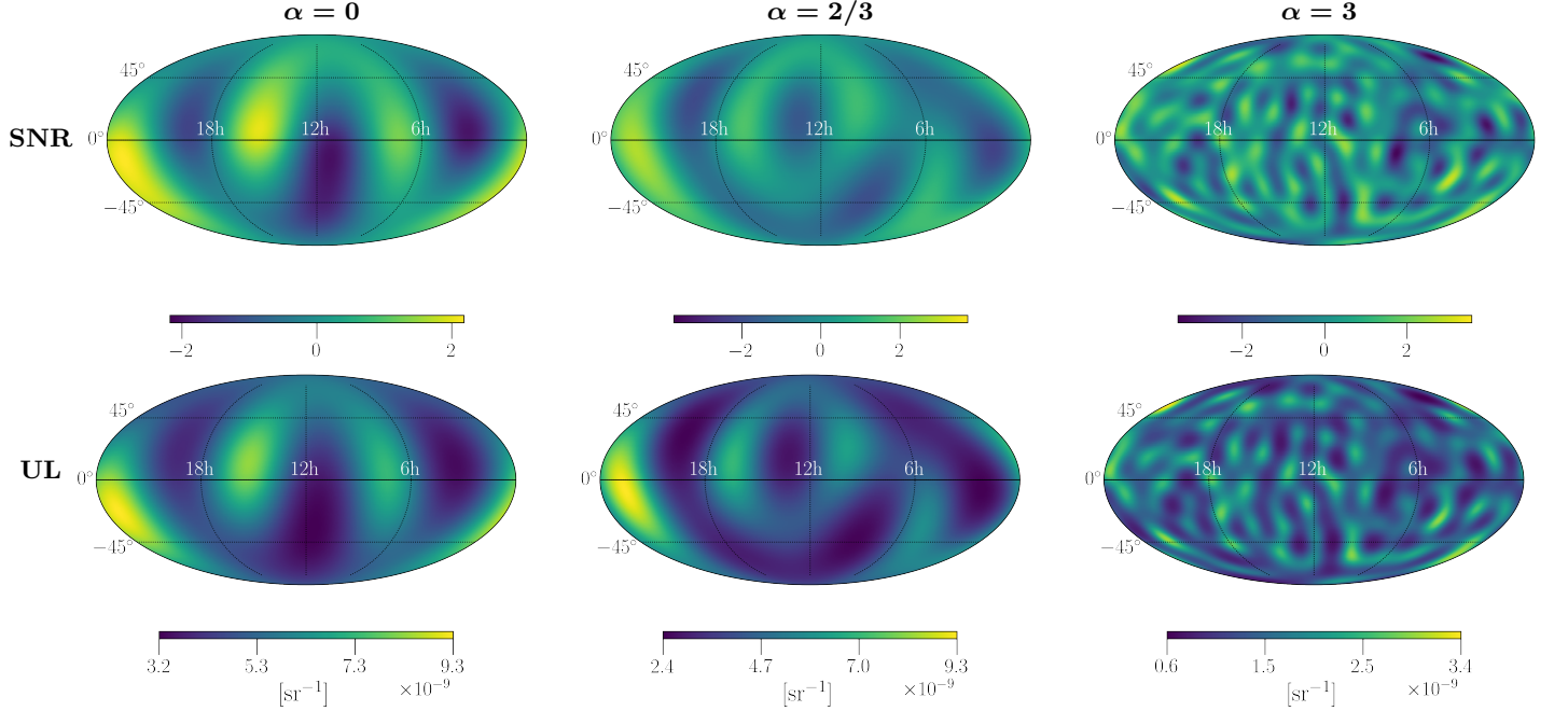
FIG. 3. Top row: SNR maps from the SHD search for extended sources. Bottom row: sky maps representing 95% upper limit on the normalized gravitational-wave energy density \Omega_\alpha(\Theta)[\text{sr}^{-1}] . Both sets of maps, presented in equatorial coordinate system, are derived by combining all three observing runs of LIGO-Virgo data (Virgo was incorporated only for O3). \alpha = 0, 2/3 , and 3 are represented from left to right.
