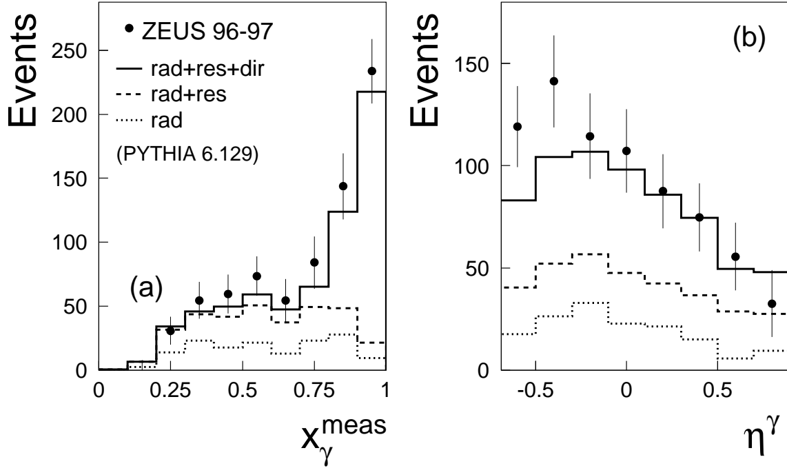
Figure 1: Distributions of (a) x_{\gamma}^{\text{meas}} , (b) photon pseudorapidity, \eta^{\gamma} , for prompt photon events in which a jet is also observed. The plotted errors are statistical only. The data are compared with predictions from PYTHIA 6.129. The PYTHIA histograms indicate contributions from dijet events where a final-state quark radiates a photon (dotted line), summed with resolved prompt photon events (dashed line), and also with direct prompt photon events (full line). The PYTHIA 6.129 default \langle k_T \rangle values in the proton and photon have been used. The Monte Carlo predictions are normalised to the integrated luminosity of the data.
