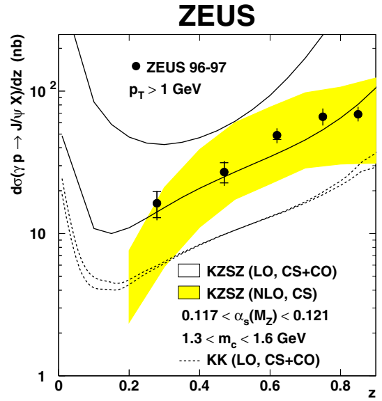
Fig. 8. Differential cross-section d\sigma/dz for 50 < W < 180 GeV and p_T > 1 GeV ( points ). The inner error bars show the statistical uncertainty; the outer bars show the statistical and systematic uncertainties added in quadrature. The shaded band shows the prediction KZSZ (NLO, CS), including only the direct photon process. The spread in the prediction is due to uncertainties on the charm-quark mass and on the QCD scale parameter, \Lambda_{QCD} . The solid lines show the prediction of the KZSZ (LO, CS+CO) calculation performed including both direct and resolved photon processes. The spread in the predictions is due to theoretical uncertainties in the extraction of the CO matrix elements. The KK (LO, CS+CO) prediction is also shown as the dashed line. The spread in the predictions is due to uncertainties in the extraction of the CO matrix elements. A 15% contribution has been added to the predictions to account for J/\psi mesons originating from \psi' cascade decays
