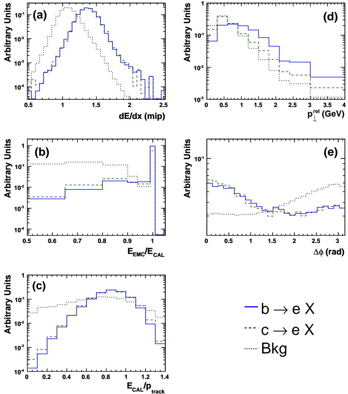
Figure 3: Normalised distributions of the five input variables used in the likelihood for the electron candidates extracted from the Monte Carlo, without applying the cuts on dE/dx and E_{EMC}/E_{CAL} . The solid line shows the distribution for electrons from semileptonic b -quark decays, the dashed line for c -quark decays and the dotted line the background (Bkg).
