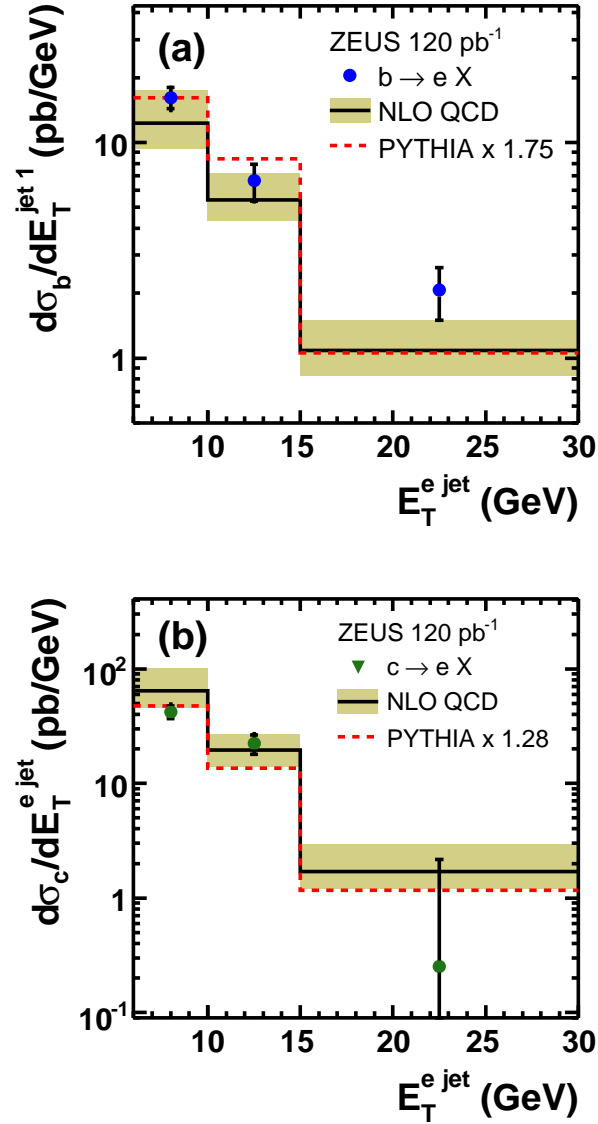
Figure 13: Differential cross sections for a) b -quark and b) c -quark production as a function of the transverse energy of the jet associated to the electron. Other details as in the caption of Fig. 10.
