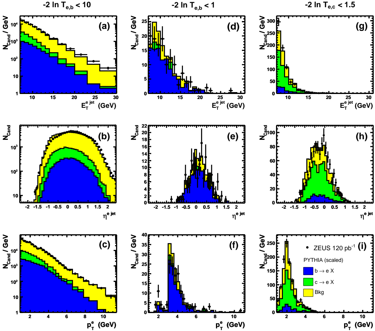
Figure 8: Distributions of E_T^{e \text{ jet}} and \eta^{e \text{ jet}} of the jet associated with the electron, and p_T^e of the electron candidate. Figures a)-c) contain all electron candidates satisfying -2 \ln T_{e,b} < 10 ; d)-f) and g)-i) show the same distributions for the beauty ( -2 \ln T_{e,b} < 1 ) and charm ( -2 \ln T_{e,c} < 1.5 ) enriched samples, respectively. Other details as in the caption of Fig. 5.
