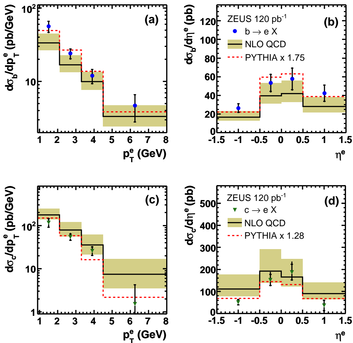
Figure 10: Differential cross sections as a function of a), c) the transverse momentum and b), d) the pseudorapidity of the electrons. Plots a) and b) are for b -quark production while c) and d) are for c -quark production. The measurements are shown as points. The inner error bar shows the statistical uncertainty and the outer error bar shows the statistical and systematic uncertainties added in quadrature. The solid line shows the NLO QCD prediction after hadronisation corrections, with the theoretical uncertainties indicated by the band; the dashed line shows the scaled prediction from PYTHIA.
