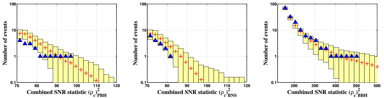
FIG. 3: Cumulative histograms of the combined SNR, \rho_c , for in-time coincident candidate events (triangles) and estimated background from accidental coincidences (crosses and 1 standard-deviation ranges), for the S4 PBH binary (left), S4 BNS (middle) and S4 BBH (right) searches. In each search, the loudest candidate (found in non-playground time) corresponds to an accidental coincidence rate of about 1 during the entire S4 run.
