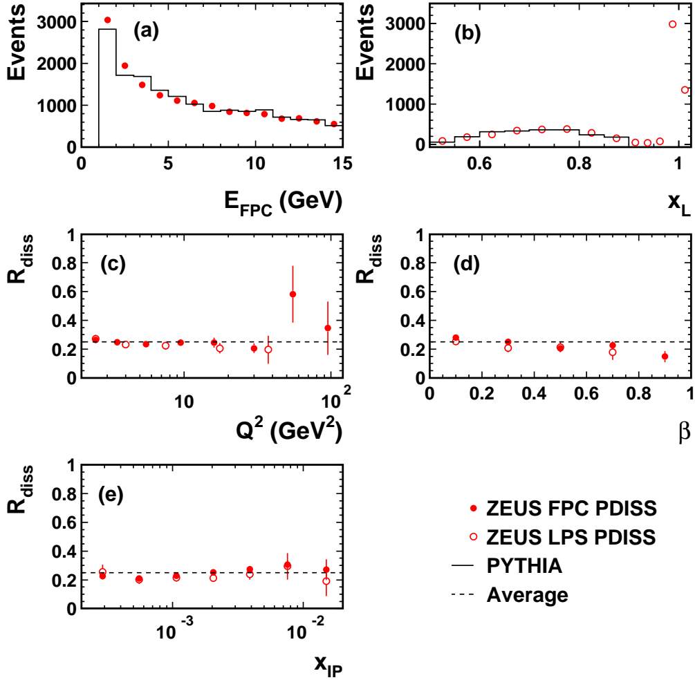
Figure 4: (a) The energy distribution in the FPC, E_{\text{FPC}} , for the sample of proton-dissociative candidate events (FPC PDISS). The data (dots) are compared to the expectation of the reweighed PYTHIA MC (histogram), normalised to the data. (b) The x_L distribution in the LPS for the sample of proton-dissociative candidate events (LPS PDISS). The data (open circles) are compared to the expectation of the reweighed PYTHIA MC (histogram), normalised to the data in the range 0.5 < x_L < 0.9 . The data points for x_L > 0.9 are also shown for completeness. The extracted fraction of proton-dissociative events, R_{\text{diss}} , from the two samples as a function of (c) Q^2 , (d) \beta and (e) x_{\text{IP}} . The dashed lines in (c), (d) and (e) represent the average of the points.
