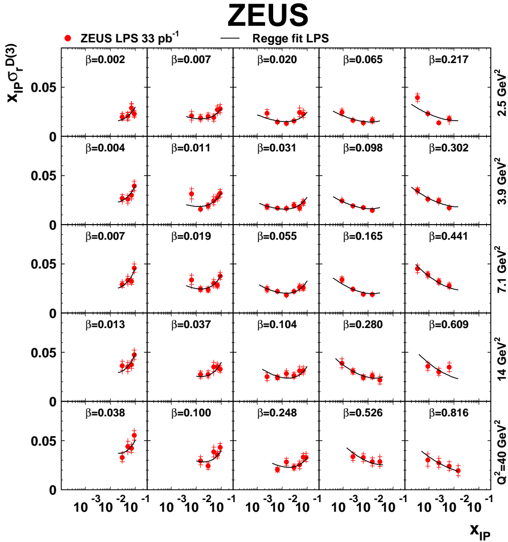
Figure 11: The reduced diffractive cross section multiplied by x_{\mathbb{P}} , x_{\mathbb{P}}\sigma_r^{D(3)} , obtained with the LPS method as a function of x_{\mathbb{P}} for different values of Q^2 and \beta . The lines are the result of the Regge fit described in Section 10.5. The inner error bars show the statistical uncertainties and the full bars indicate the statistical and the systematic uncertainties added in quadrature. The normalisation uncertainty of {}_{-7}^{+11}\% is not shown.
