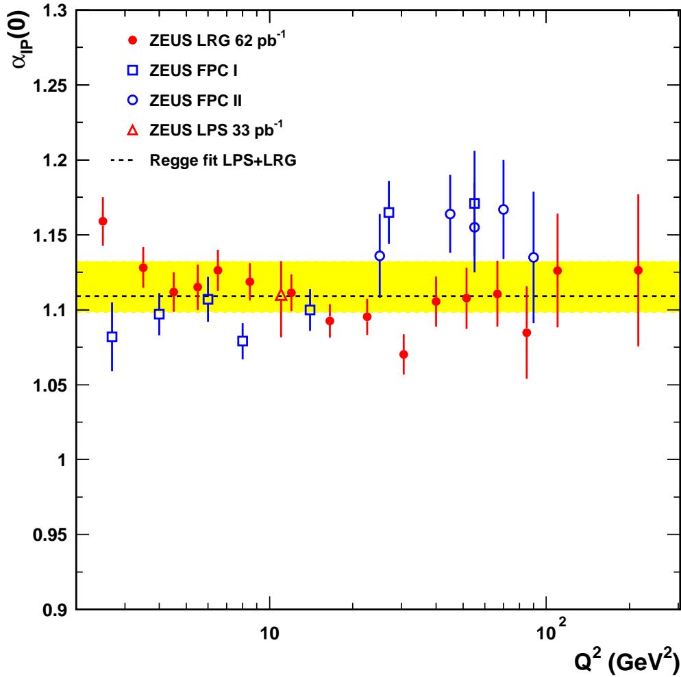
Figure 21: The Pomeron intercept \alpha_{\mathbb{P}}(0) as a function of Q^2 as obtained from the LRG (dots) and the LPS data (triangles). Also shown are the M_X -method results, FPC I (open squares) and FPC II (open circles). The error bars indicate the uncertainty from the fit for the LRG and FPC points; they indicate the statistical and systematic uncertainties summed in quadrature for the LPS points. The dashed line indicates the results of the Regge fit to the LPS and LRG data together described in Section 10.5, and the band indicates the size of the total error.
