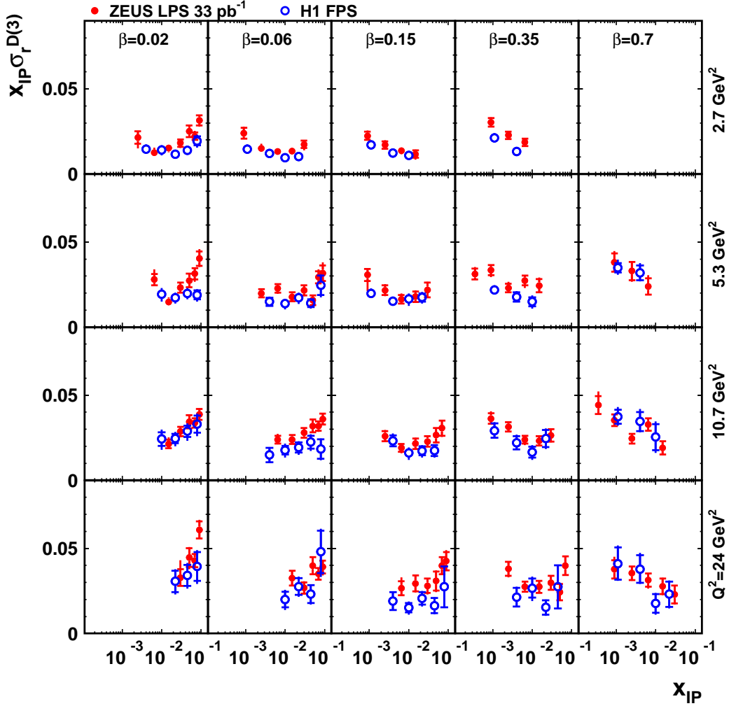
Figure 12: The reduced diffractive cross section multiplied by x_{\mathcal{P}} , x_{\mathcal{P}}\sigma_r^{D(3)} , obtained with the LPS method (dots) as a function of x_{\mathcal{P}} for different values of Q^2 and \beta compared with the results obtained with the H1 Forward Proton Spectrometer (open circles). The inner error bars show the statistical uncertainties and the full bars indicate the statistical and the systematic uncertainties added in quadrature. The normalisation uncertainty of {}^{+11}_{-7}\% of the ZEUS data is not shown, nor is that of the H1 data ( \pm 10\% ).
