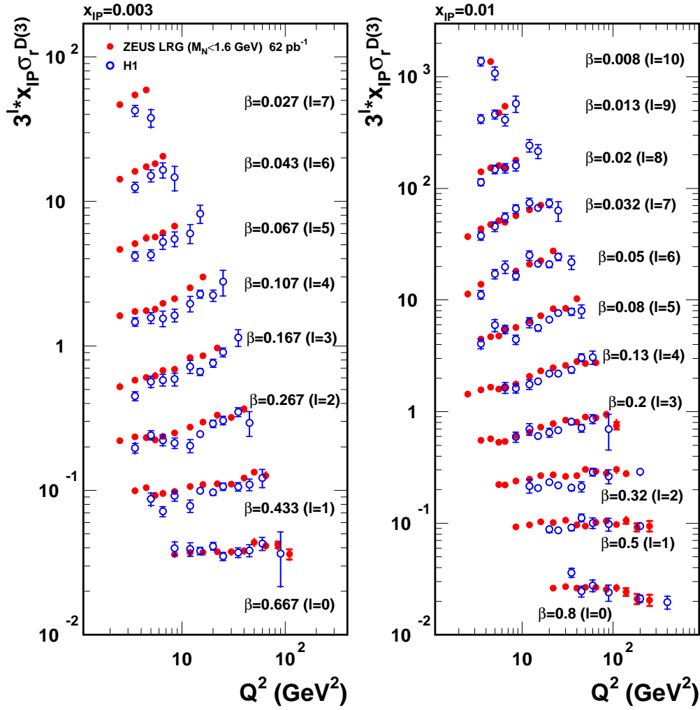
Figure 17: The reduced diffractive cross section multiplied by x_P , x_P \sigma_r^{D(3)} , obtained with the LRG method (dots) at x_P = 0.003 and x_P = 0.01 as a function of Q^2 for different \beta values compared with the H1 results (open circles), also obtained with the LRG method. Other details as in caption for Fig. 16.
