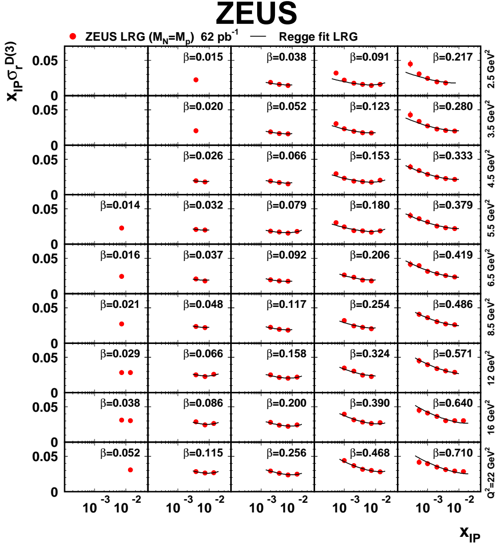
Figure 13: The reduced diffractive cross section multiplied by x_{\mathbb{P}} , x_{\mathbb{P}}\sigma_r^{D(3)} , obtained with the LRG method as a function of x_{\mathbb{P}} for different values of Q^2 and \beta at low Q^2 values. The lines are the result of the Regge fit described in Section 10.5. The inner error bars show the statistical uncertainties and the full bars indicate the statistical and the systematic uncertainties added in quadrature. The data are corrected for the proton-dissociative background to M_N = M_p as described in Section 8.1. The normalisation uncertainty of \pm 5\% is not shown.
