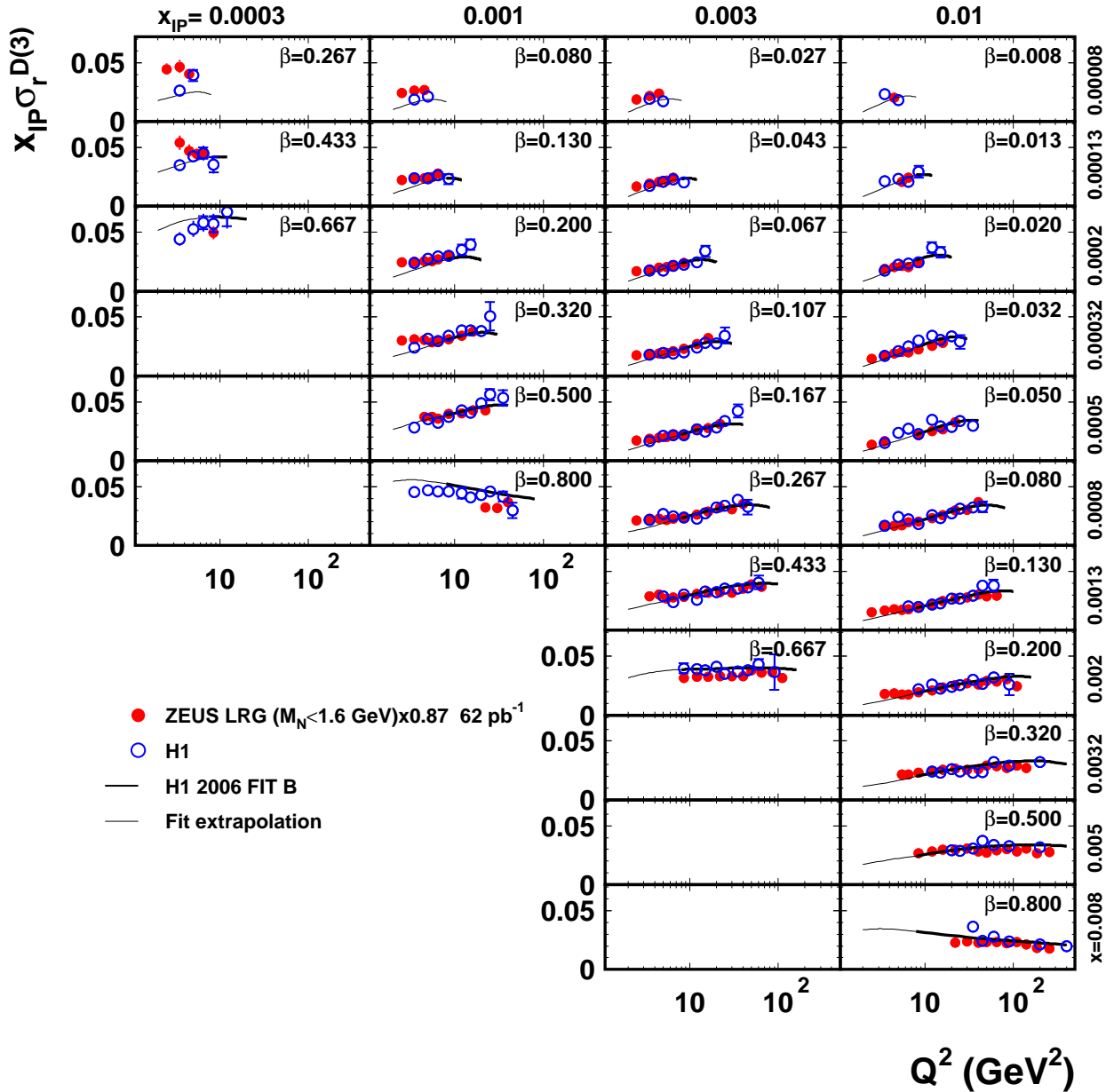
Figure 18: The reduced diffractive cross section multiplied by x_P , x_P \sigma_r^{D(3)} , obtained with the LRG method (dots) as a function of Q^2 for different \beta and x_P values compared with the H1 results (open circles), also obtained with the LRG method. The lines represent the expectation based on the diffractive parton distribution functions “H1 2006 fit B”. The inner error bars show the statistical uncertainties and the full bars indicate the statistical and the systematic uncertainties added in quadrature. The ZEUS data are normalised to the H1 data.
