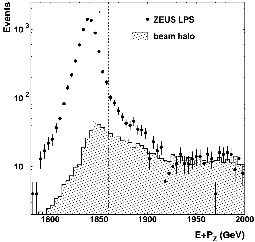
Figure 5: Distribution of E+P_Z for the LPS events (dots). The dashed histogram represents the estimate of the beam-halo background normalised for E + P_Z > 1925 GeV. The vertical dashed line at E + P_Z = 1860 GeV represents the selection cut used in the analysis.
