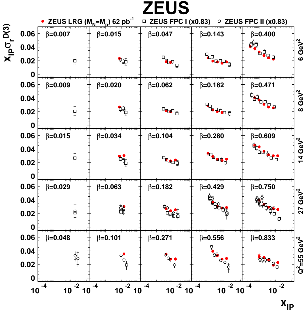
Figure 19: The reduced diffractive cross section multiplied by x_{\text{IP}} , x_{\text{IP}} \sigma_r^{D(3)} , obtained with the LRG method (dots) as a function of x_{\text{IP}} for different values of Q^2 and \beta at low Q^2 , compared with the results obtained with the M_X method, FPC I (open squares) and FPC II (open circles), scaled by the factor 0.83 described in Section 10.4. The inner error bars show the statistical uncertainties and the full bars indicate the statistical and the systematic uncertainties added in quadrature.
