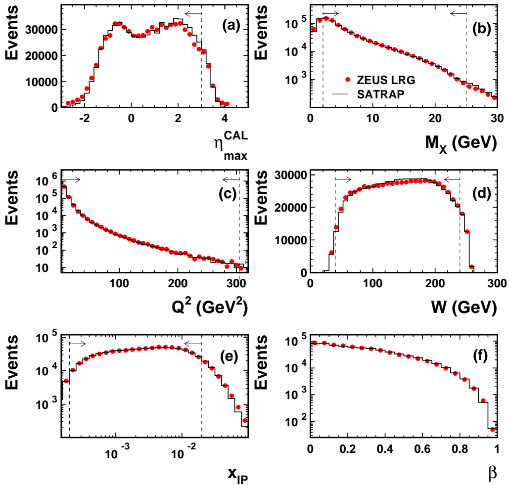
Figure 2: Comparison of the distributions measured (dots) and obtained with the reweighted SATRAP MC (histograms) for (a) \eta_{\max}^{\text{CAL}} , (b) M_X , (c) Q^2 , (d) W , (e) x_{\text{IP}} and (f) \beta in the LRG analysis. For each plot, all analysis cuts have been applied except that on the plotted variable. The vertical lines with arrows indicate the selected region.
