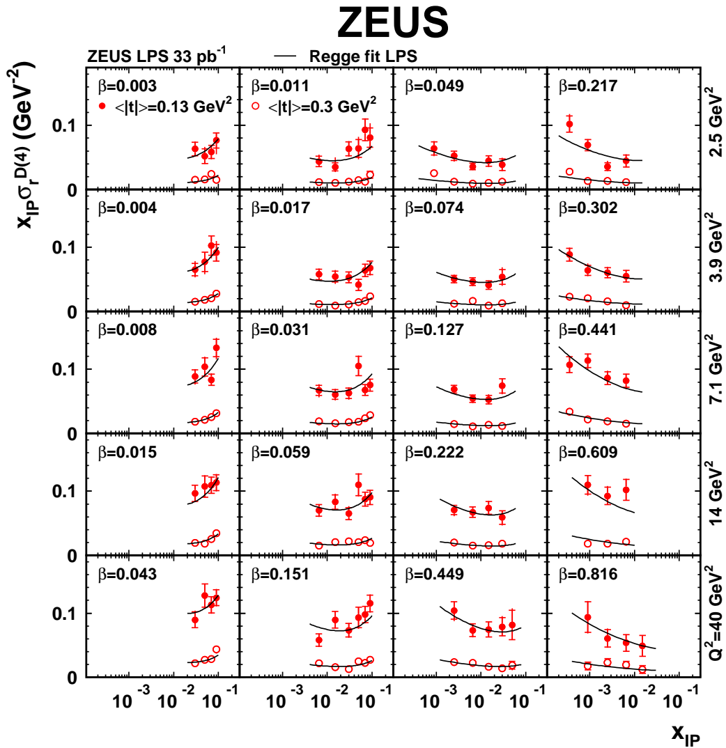
Figure 10: The reduced diffractive cross section multiplied by x_{\mathbb{P}} , x_{\mathbb{P}} \sigma_r^{D(4)} , obtained with the LPS method in two t bins as a function of x_{\mathbb{P}} for different values of Q^2 and \beta . The lines are the result of the Regge fit described in Section 10.5. The inner error bars show the statistical uncertainties and the full bars indicate the statistical and the systematic uncertainties added in quadrature. The normalisation uncertainty of \pm 7\% is not shown.
